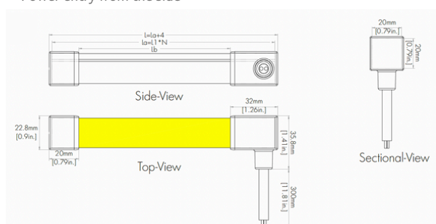
Power entry from the side
